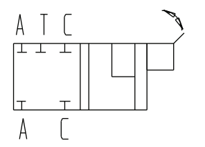
FUNCTIONAL SYMBOL
