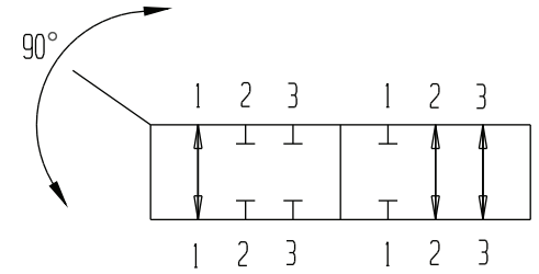
FUNCTION DIAGRAM
