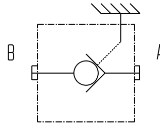
FUNCTIONAL SYMBOL
