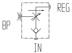
FUNCTIONAL SYMBOL
