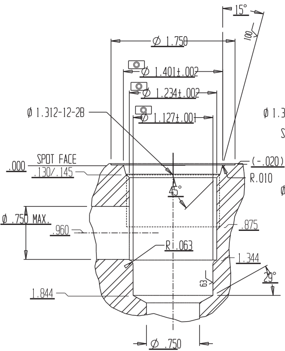
CAVITY 5053-16-2
