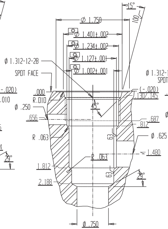
CAVITY 5053-16-3S
