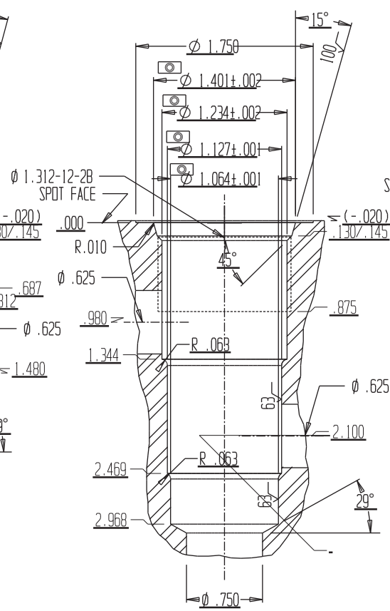
CAVITY 5053-16-3
